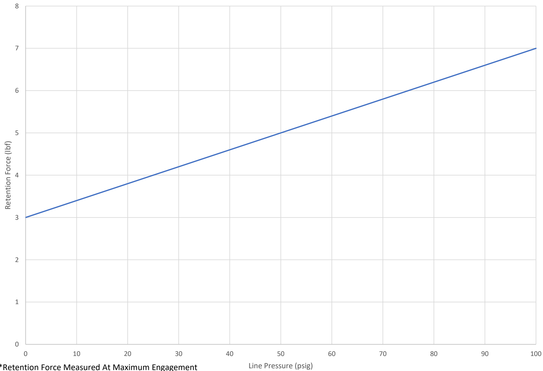
Q1NL Retention Force* vs. Line Pressure
