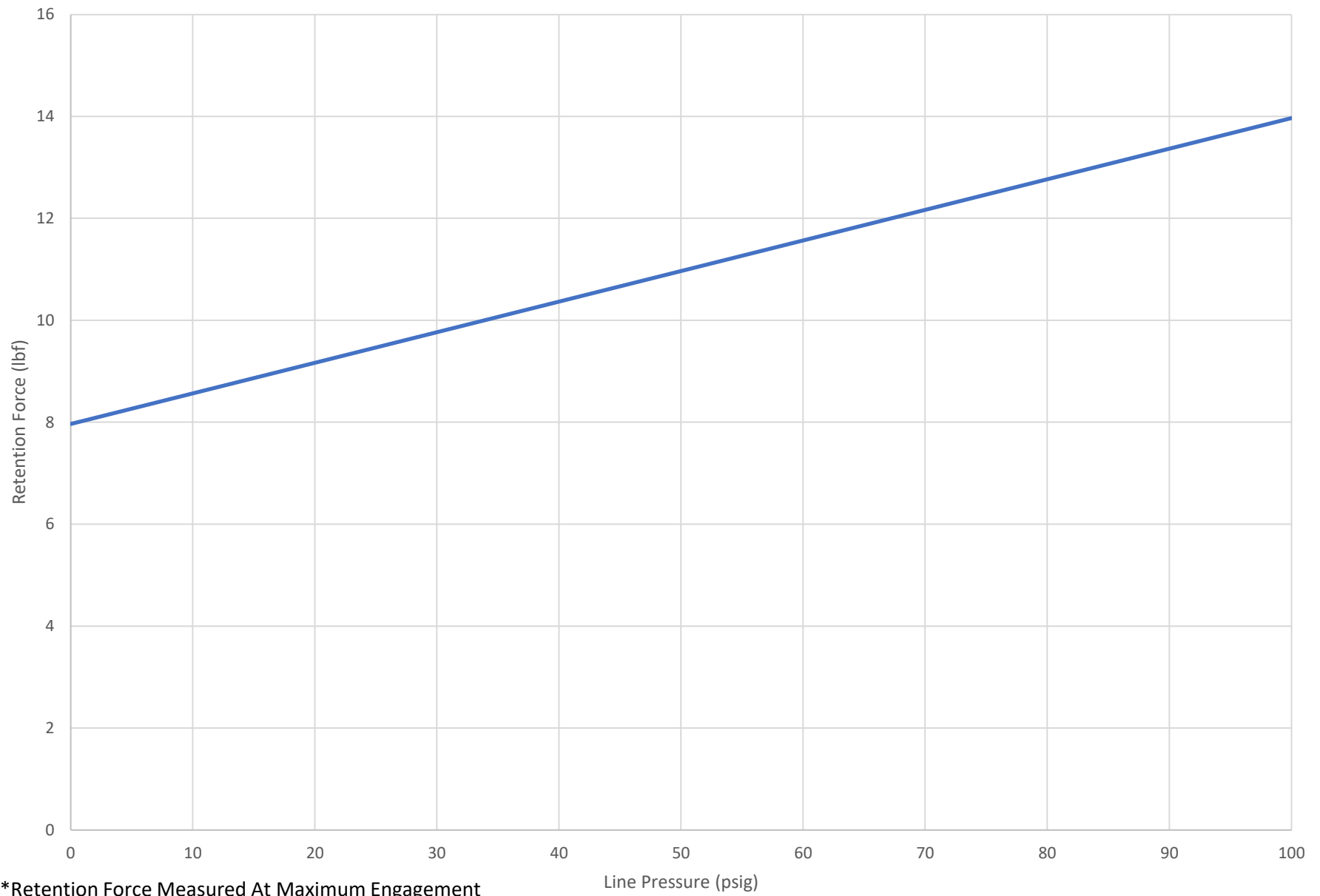
QD3NL Retention Force* vs. Line Pressure
