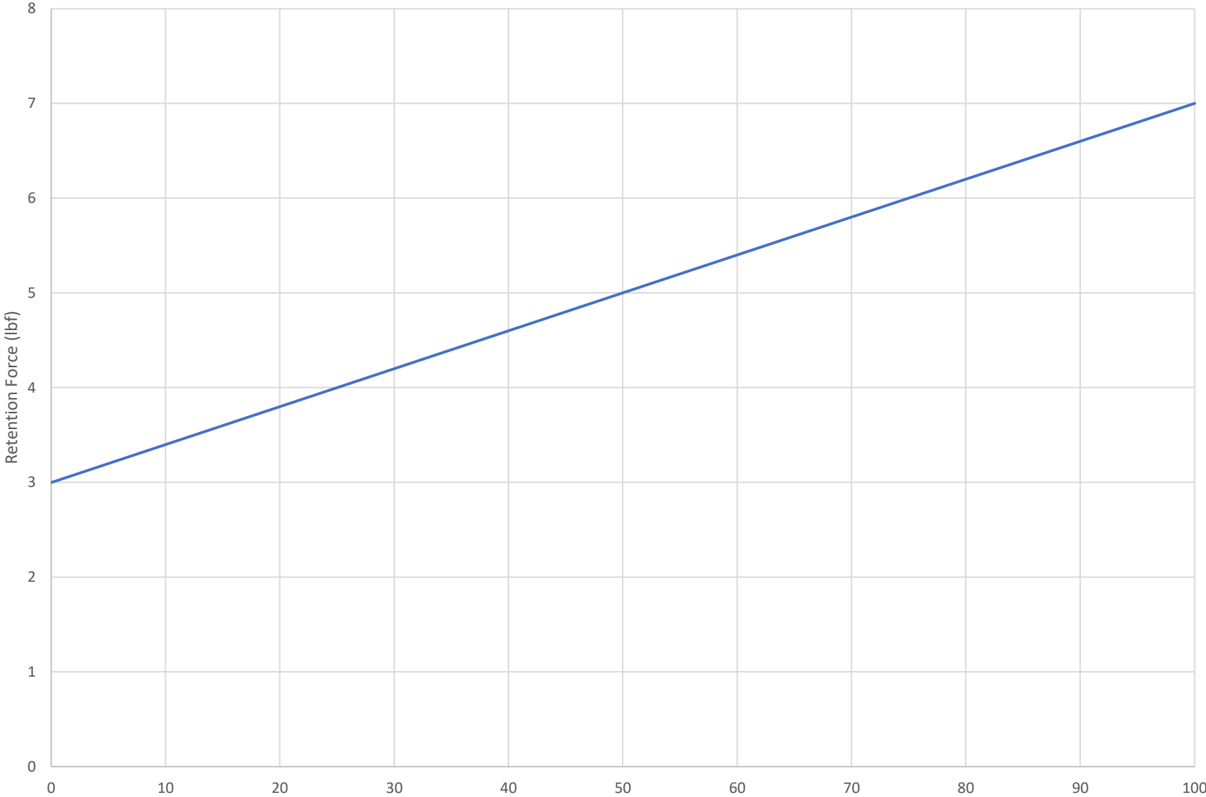
QDNL Retention Force* vs. Line Pressure
