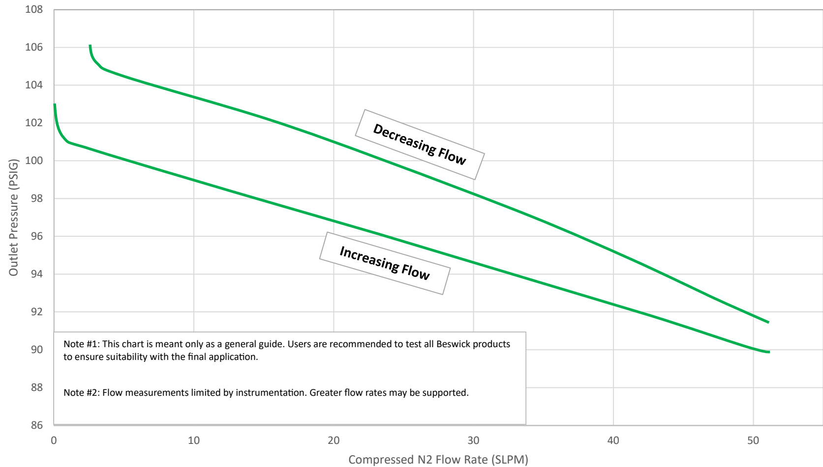
PR3HP-7N1 flow curve, inlet pressure: 2500 PSIG
