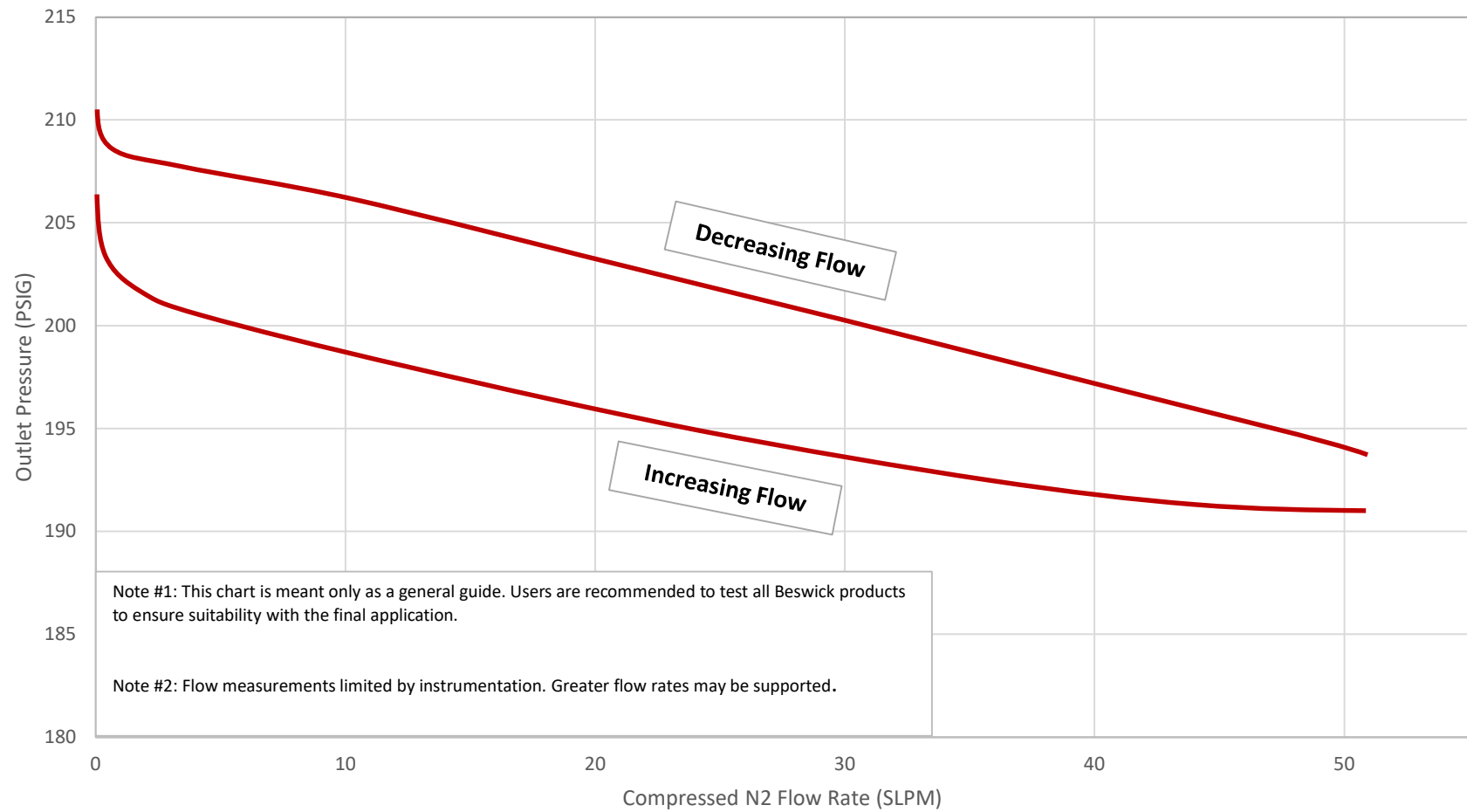
PR3HP-7N1 flow curve, inlet pressure: 2500 PSIG
