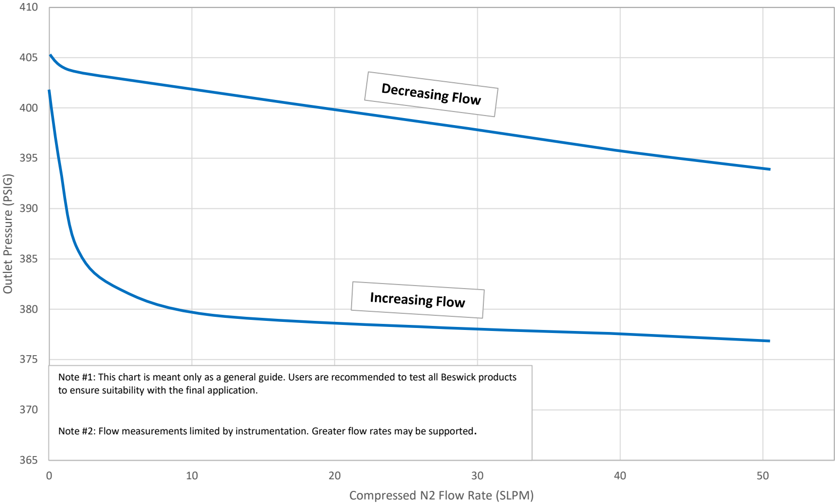
PR3HP-7N1 flow curve, inlet pressure: 2500 PSIG
